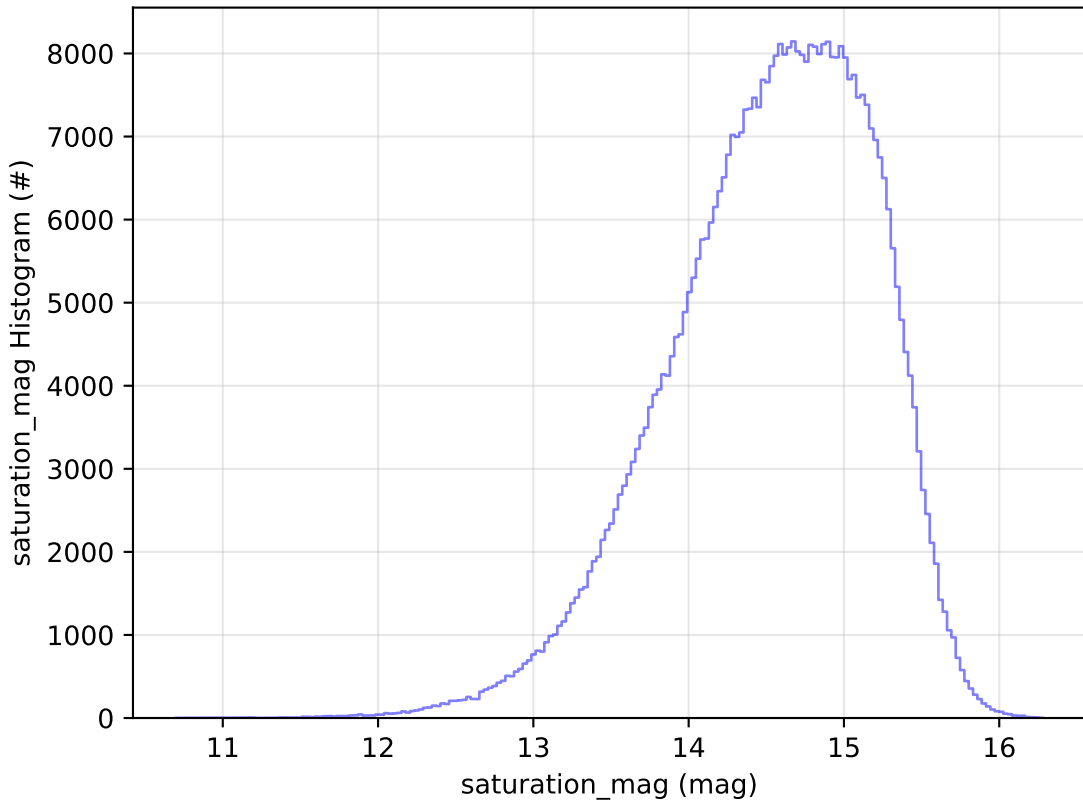
early_u_fpextra3.0_v3.4_10yrs All sky r band: saturation_mag Histogram
