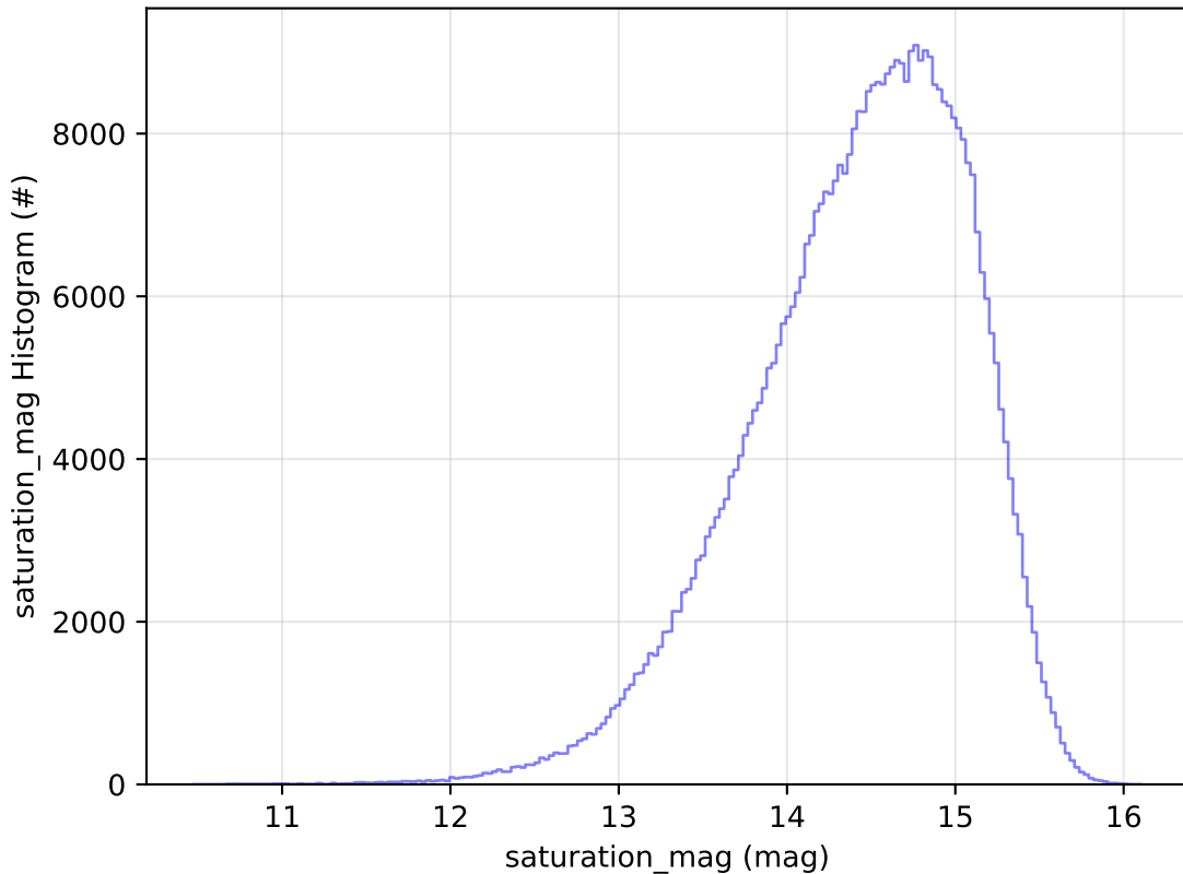
early_u_fpextra3.0_v3.4_10yrs All sky i band: saturation_mag Histogram
