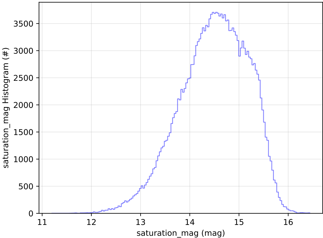
early_u_fpextra3.0_v3.4_10yrs All sky g band: saturation_mag Histogram
