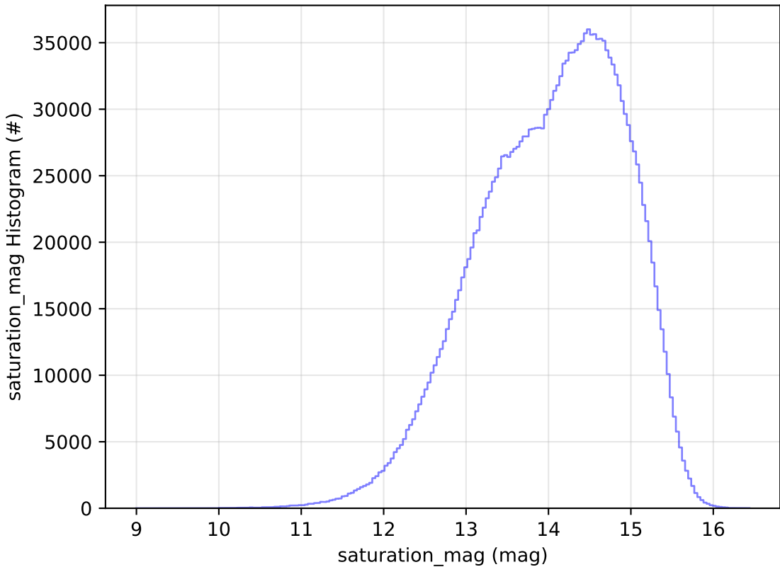
early_u_fpextra3.0_v3.4_10yrs All sky all bands: saturation_mag Histogram
