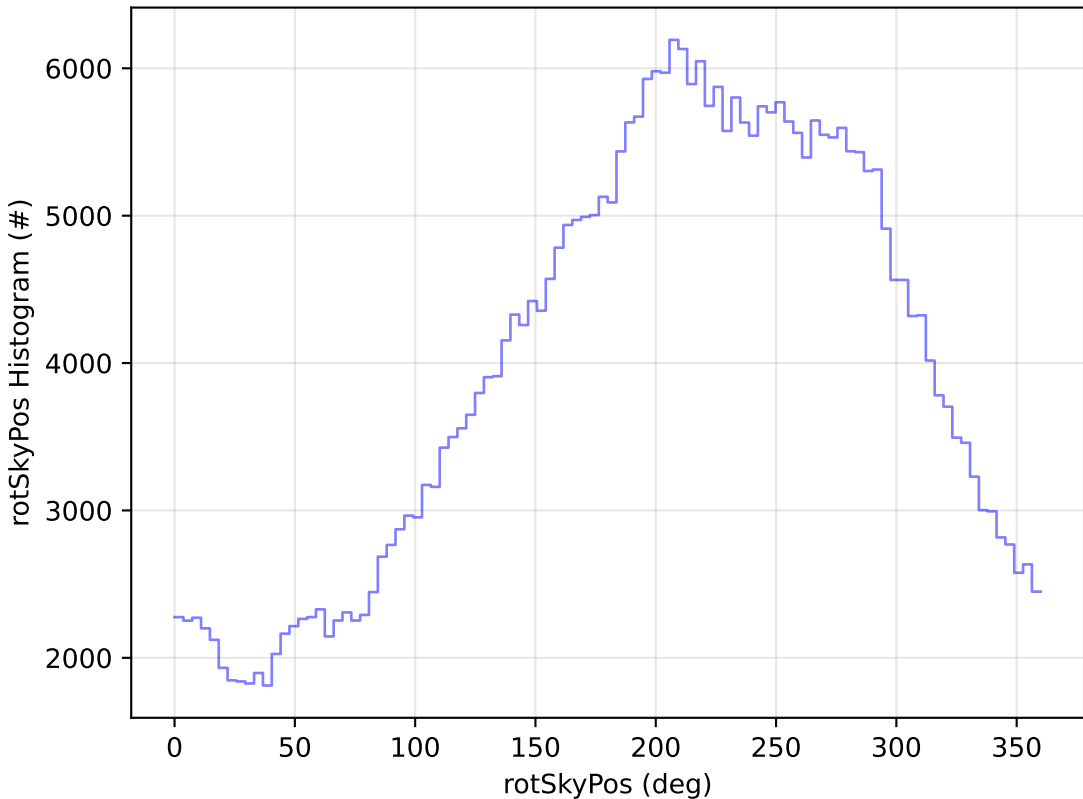
early_u_fpextra3.0_v3.4_10yrs WFD y band: rotSkyPos Histogram
