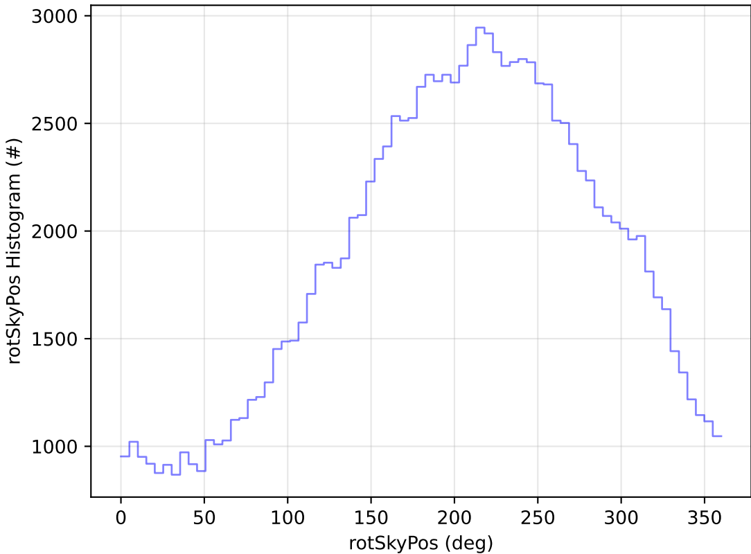
early_u_fpextra3.0_v3.4_10yrs WFD u band: rotSkyPos Histogram
