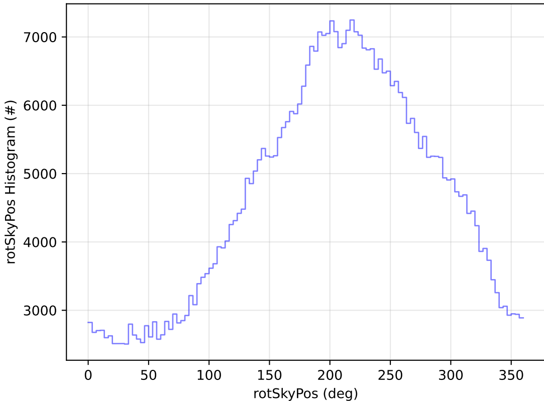
early_u_fpextra3.0_v3.4_10yrs WFD i band: rotSkyPos Histogram
