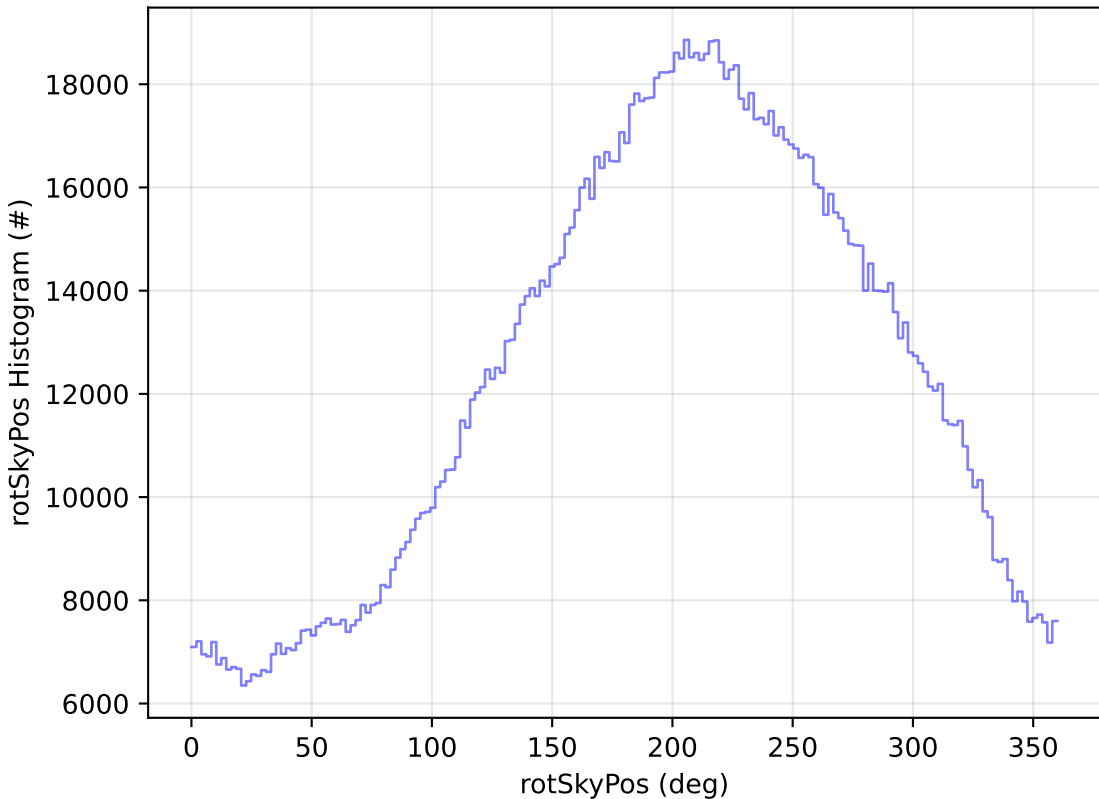
early_u_fpextra3.0_v3.4_10yrs WFD all bands: rotSkyPos Histogram
