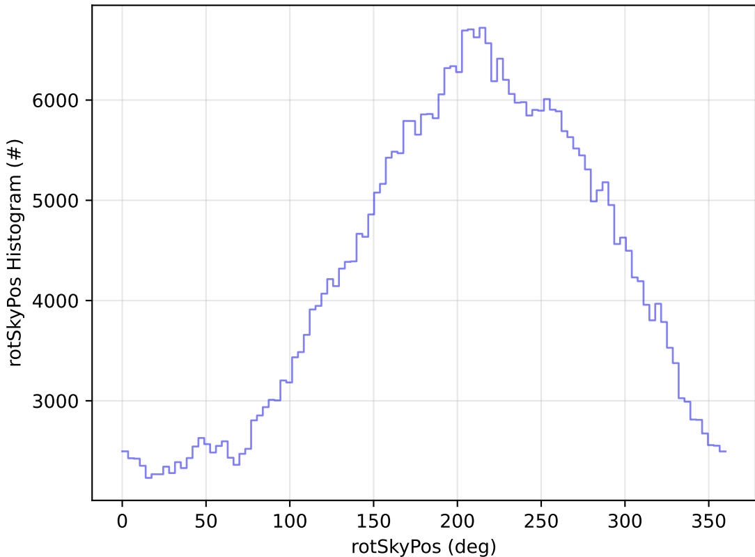
early_u_fpextra3.0_v3.4_10yrs All sky z band: rotSkyPos Histogram
