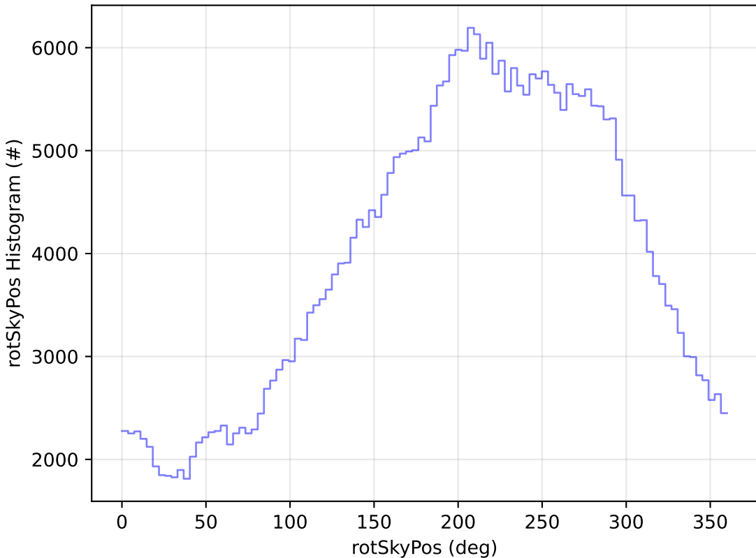
early_u_fpextra3.0_v3.4_10yrs All sky y band: rotSkyPos Histogram
