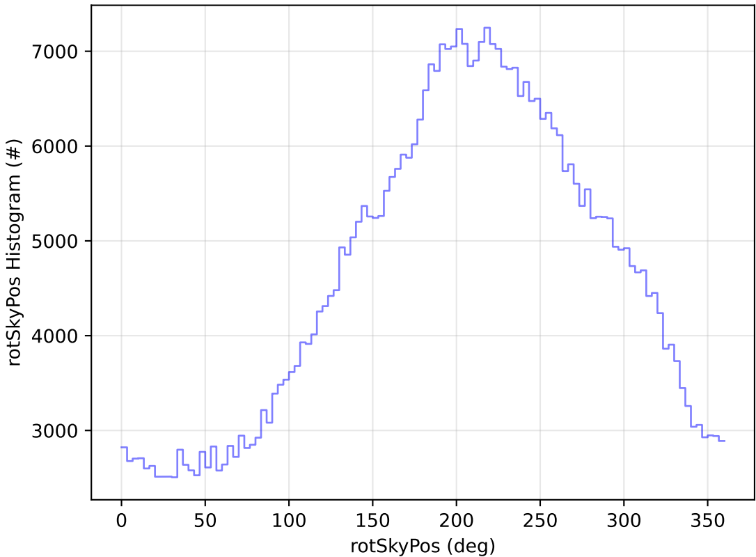
early_u_fpextra3.0_v3.4_10yrs All sky i band: rotSkyPos Histogram
