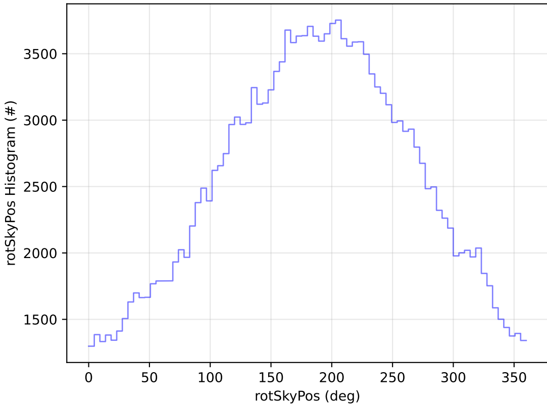
early_u_fpextra3.0_v3.4_10yrs All sky g band: rotSkyPos Histogram
