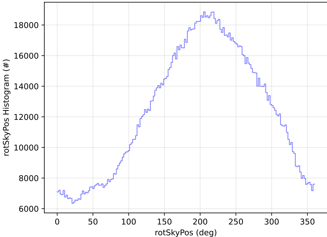
early_u_fpextra3.0_v3.4_10yrs All sky all bands: rotSkyPos Histogram
