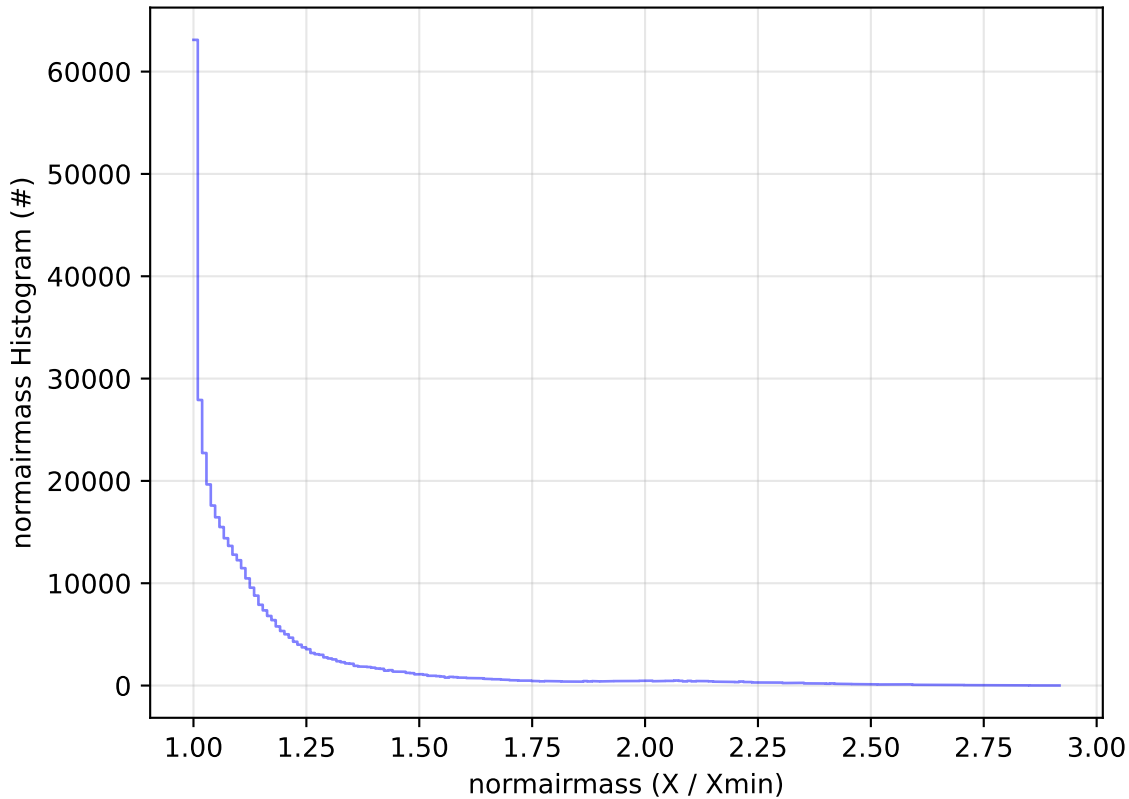
early_u_fpextra3.0_v3.4_10yrs WFD z band: normairmass Histogram
