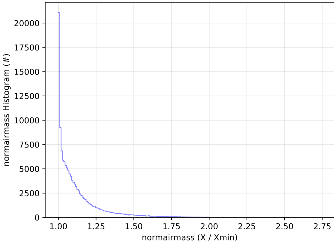
early_u_fpextra3.0_v3.4_10yrs WFD u band: normairmass Histogram
