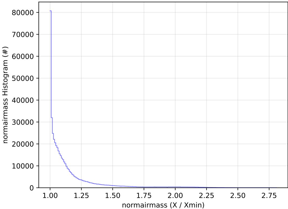
early_u_fpextra3.0_v3.4_10yrs WFD r band: normairmass Histogram
