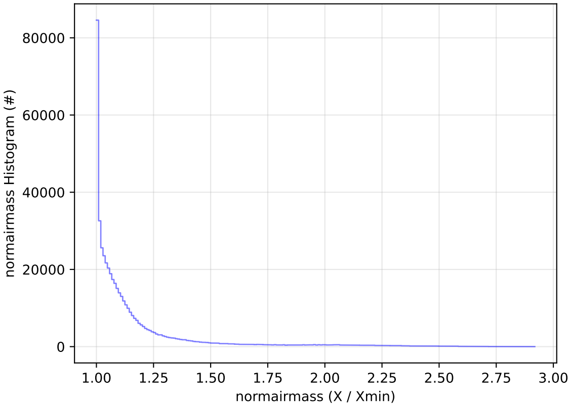
early_u_fpextra3.0_v3.4_10yrs WFD i band: normairmass Histogram
