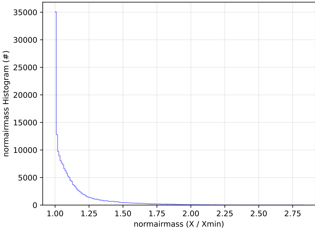
early_u_fpextra3.0_v3.4_10yrs WFD g band: normairmass Histogram
