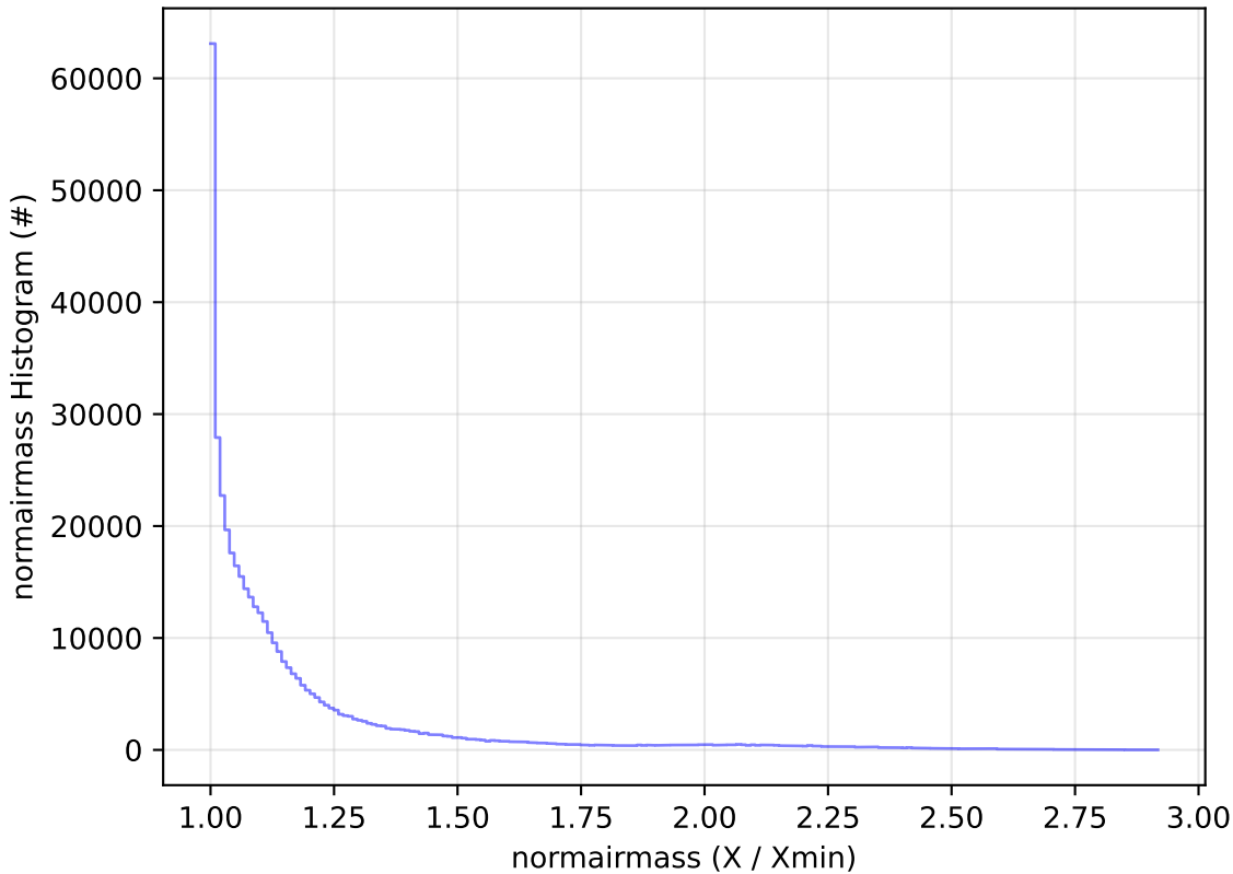
early_u_fpextra3.0_v3.4_10yrs All sky z band: normairmass Histogram
