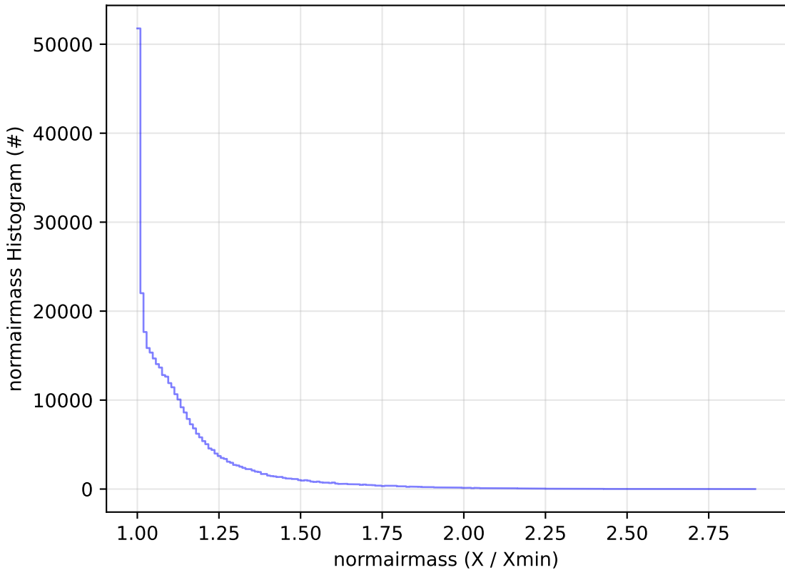
early_u_fpextra3.0_v3.4_10yrs All sky y band: normairmass Histogram
