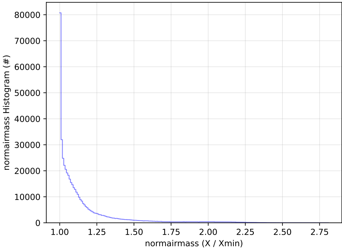
early_u_fpextra3.0_v3.4_10yrs All sky r band: normairmass Histogram
