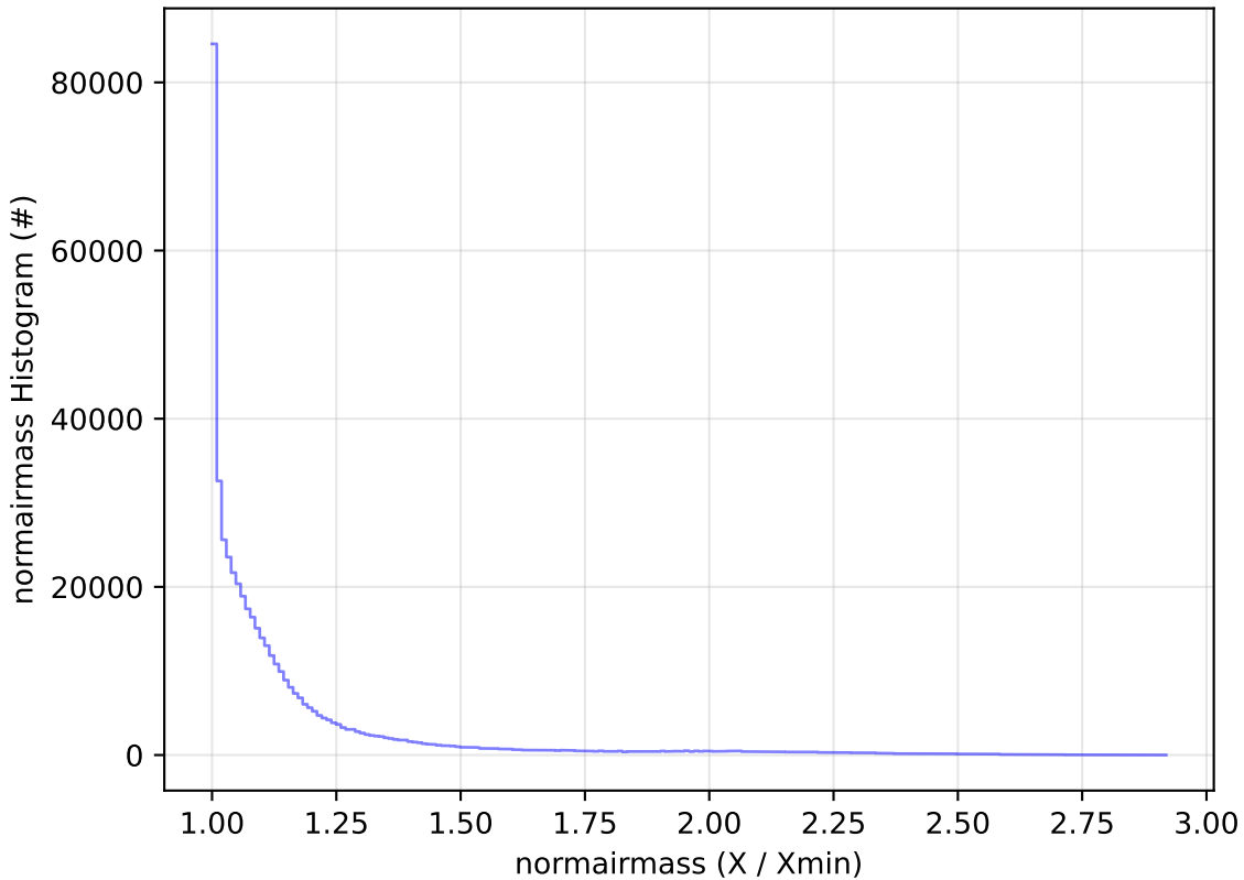
early_u_fpextra3.0_v3.4_10yrs All sky i band: normairmass Histogram
