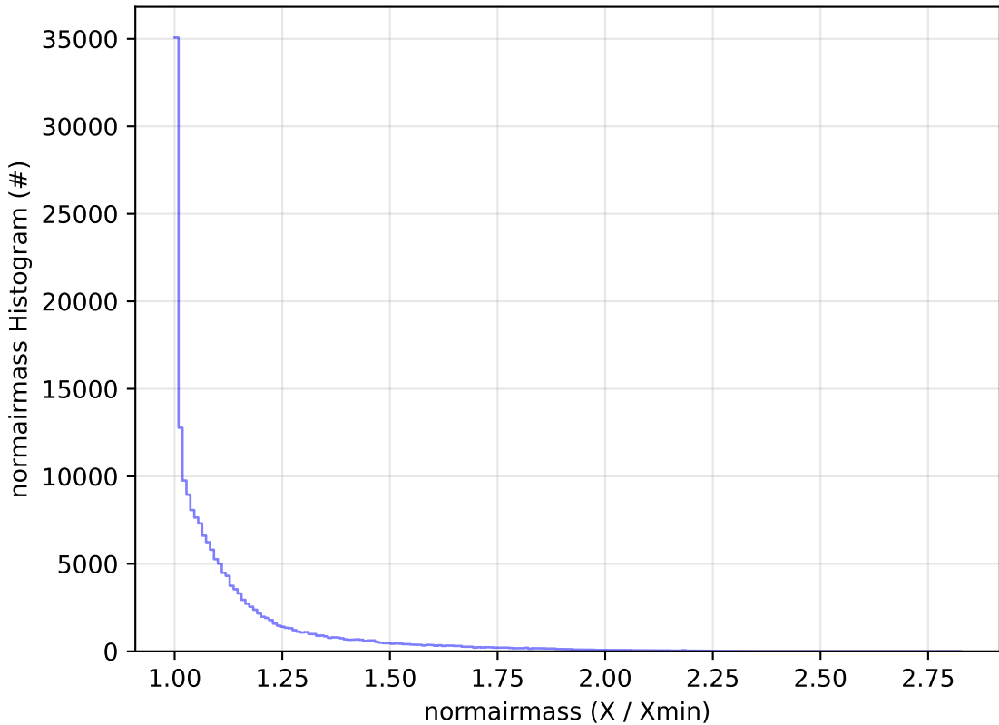
early_u_fpextra3.0_v3.4_10yrs All sky g band: normairmass Histogram
