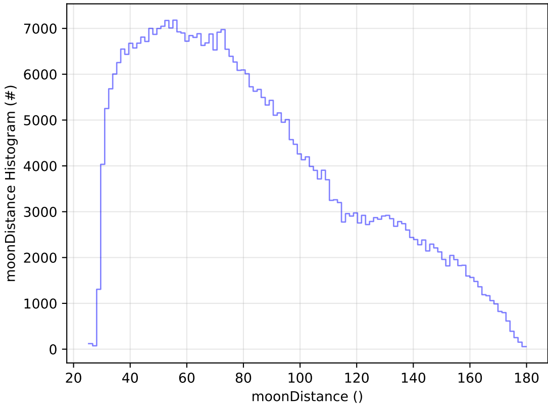
early_u_fpextra3.0_v3.4_10yrs WFD z band: moonDistance Histogram
