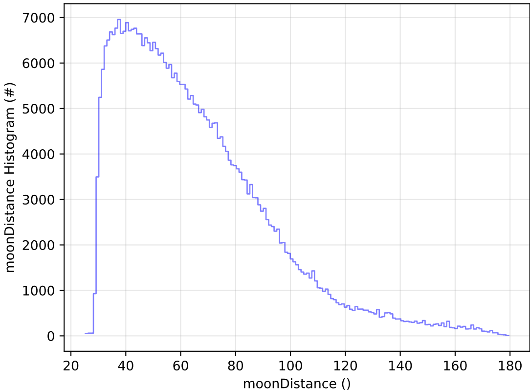
early_u_fpextra3.0_v3.4_10yrs WFD y band: moonDistance Histogram
