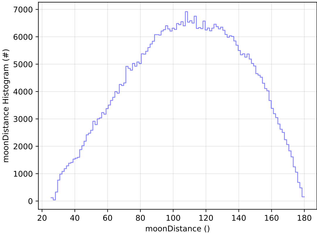
early_u_fpextra3.0_v3.4_10yrs WFD r band: moonDistance Histogram
