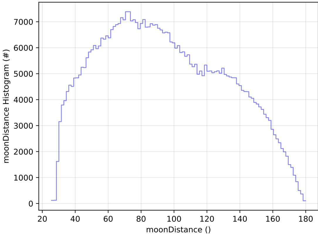
early_u_fpextra3.0_v3.4_10yrs WFD i band: moonDistance Histogram
