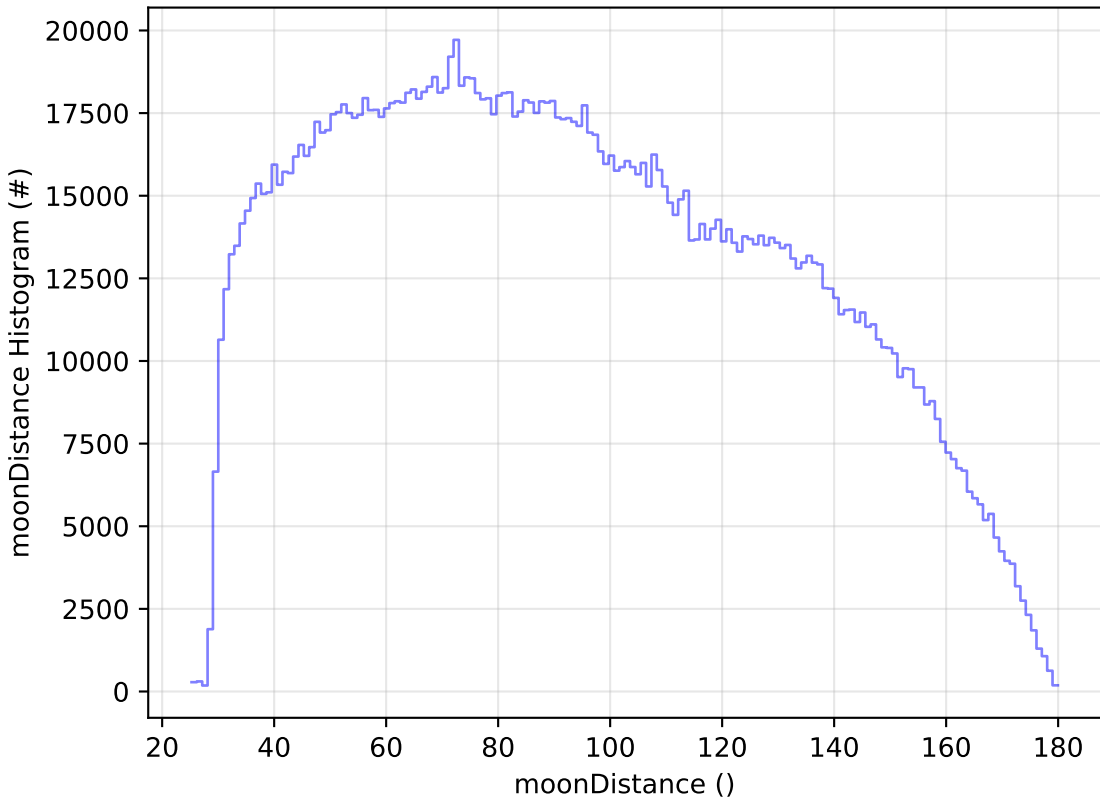
early_u_fpextra3.0_v3.4_10yrs WFD all bands: moonDistance Histogram
