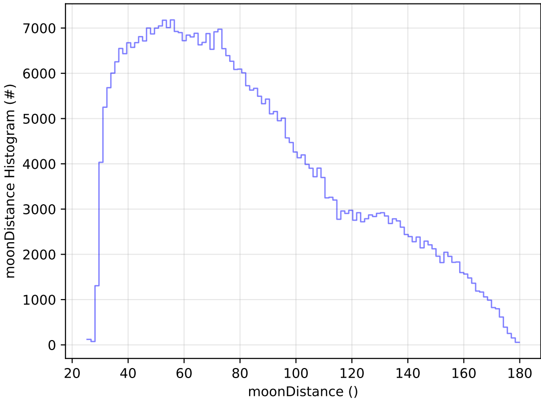
early_u_fpextra3.0_v3.4_10yrs All sky z band: moonDistance Histogram
