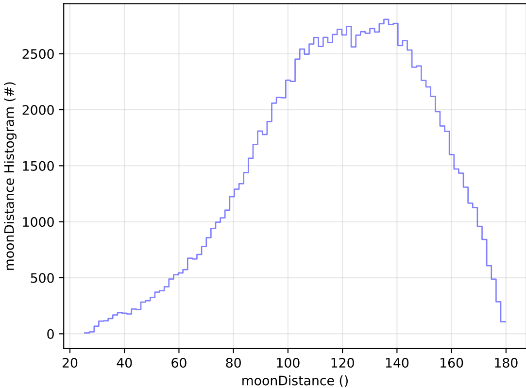
early_u_fpextra3.0_v3.4_10yrs All sky u band: moonDistance Histogram
