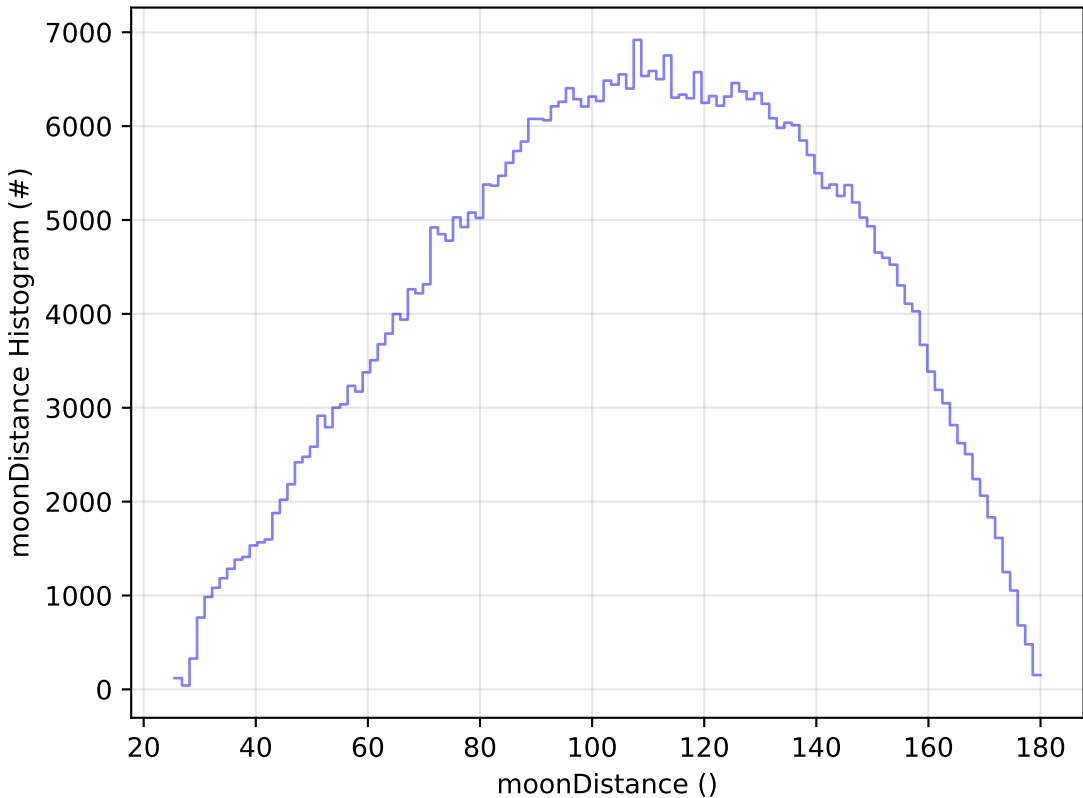
early_u_fpextra3.0_v3.4_10yrs All sky r band: moonDistance Histogram
