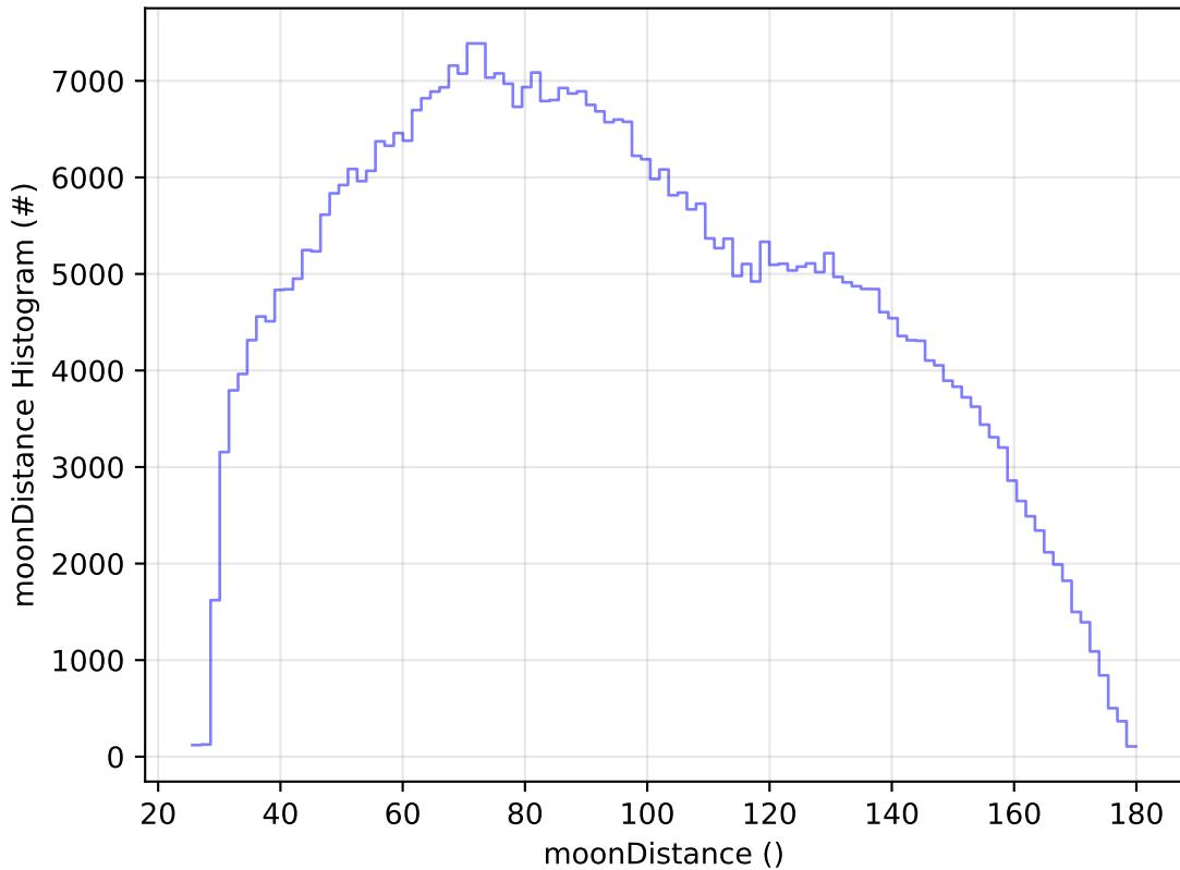
early_u_fpextra3.0_v3.4_10yrs All sky i band: moonDistance Histogram
