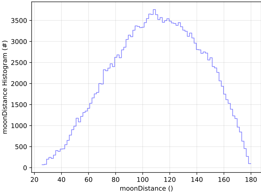
early_u_fpextra3.0_v3.4_10yrs All sky g band: moonDistance Histogram
