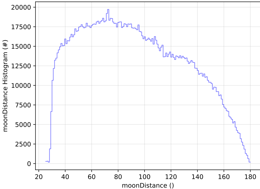
early_u_fpextra3.0_v3.4_10yrs All sky all bands: moonDistance Histogram
