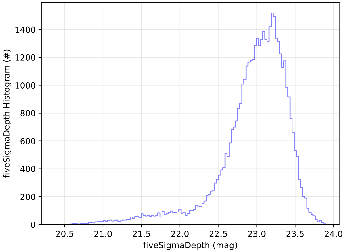
early_u_fpextra3.0_v3.4_10yrs Yr 1 z band: fiveSigmaDepth Histogram
