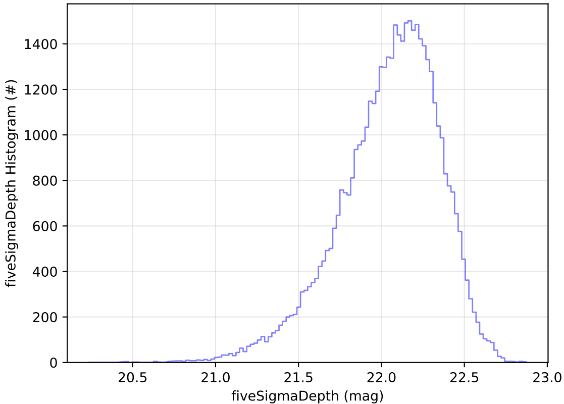
early_u_fpextra3.0_v3.4_10yrs Yr 1 y band: fiveSigmaDepth Histogram
