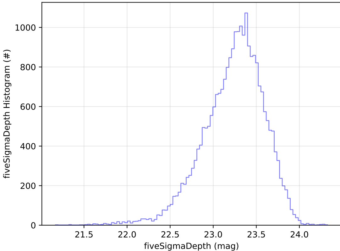
early_u_fpextra3.0_v3.4_10yrs Yr 1 u band: fiveSigmaDepth Histogram
