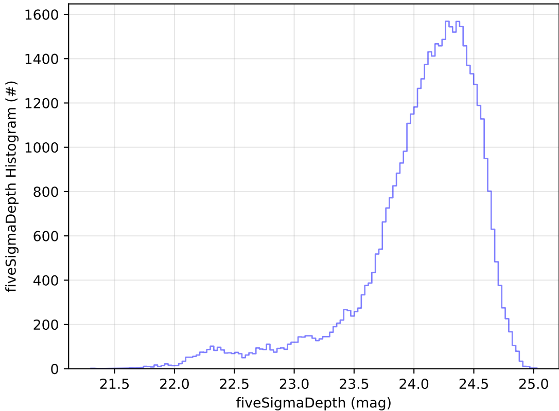
early_u_fpextra3.0_v3.4_10yrs Yr 1 r band: fiveSigmaDepth Histogram
