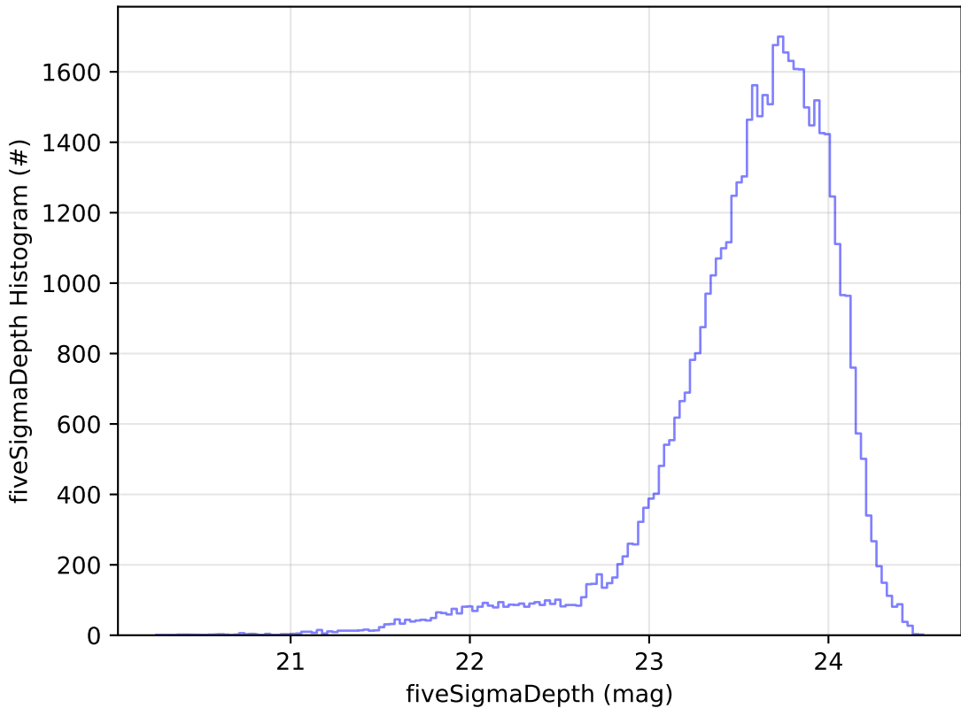
early_u_fpextra3.0_v3.4_10yrs Yr 1 i band: fiveSigmaDepth Histogram
