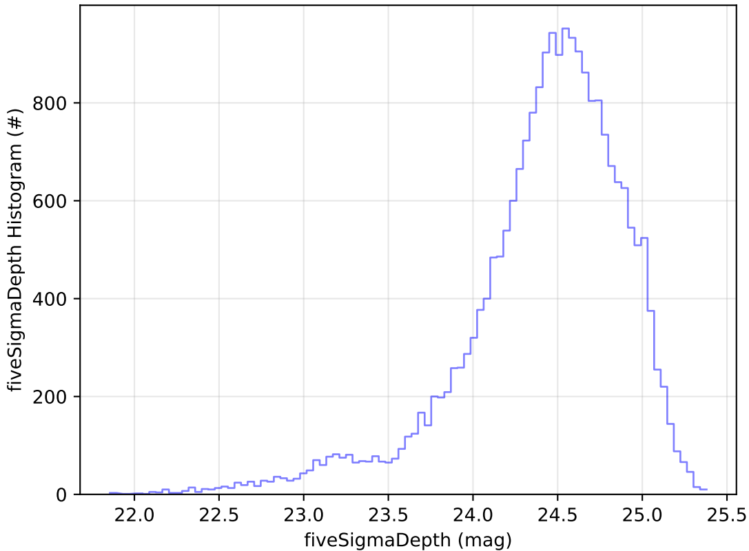
early_u_fpextra3.0_v3.4_10yrs Yr 1 g band: fiveSigmaDepth Histogram
