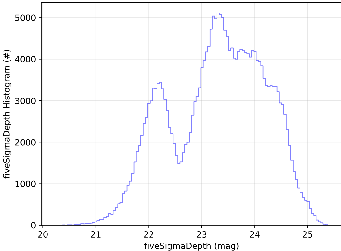
early_u_fpextra3.0_v3.4_10yrs Yr 1 all bands: fiveSigmaDepth Histogram
