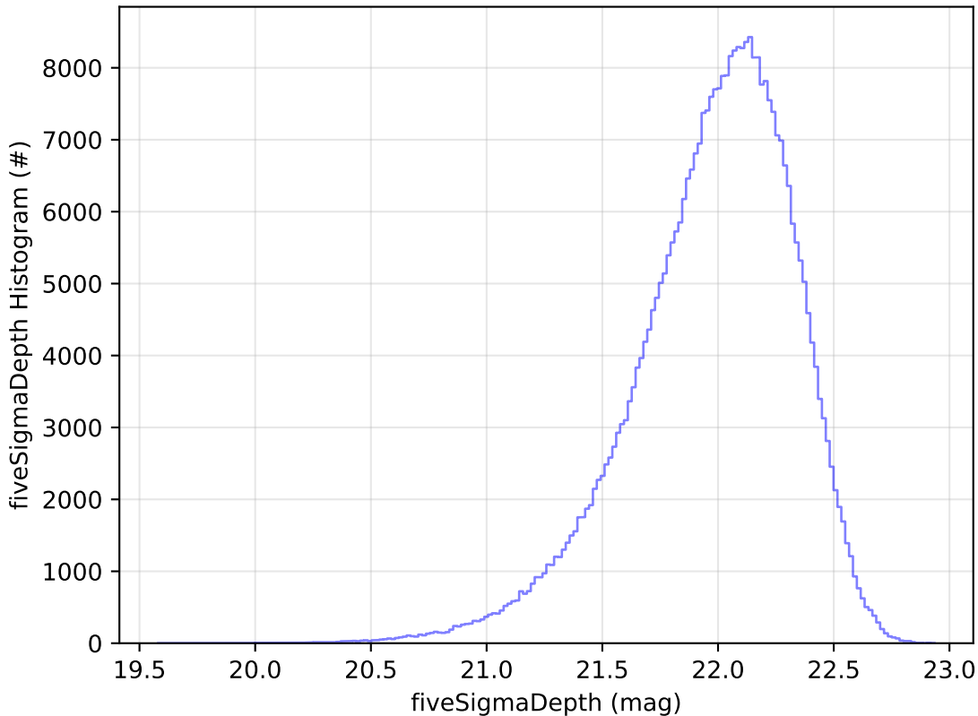
early_u_fpextra3.0_v3.4_10yrs WFD y band: fiveSigmaDepth Histogram
