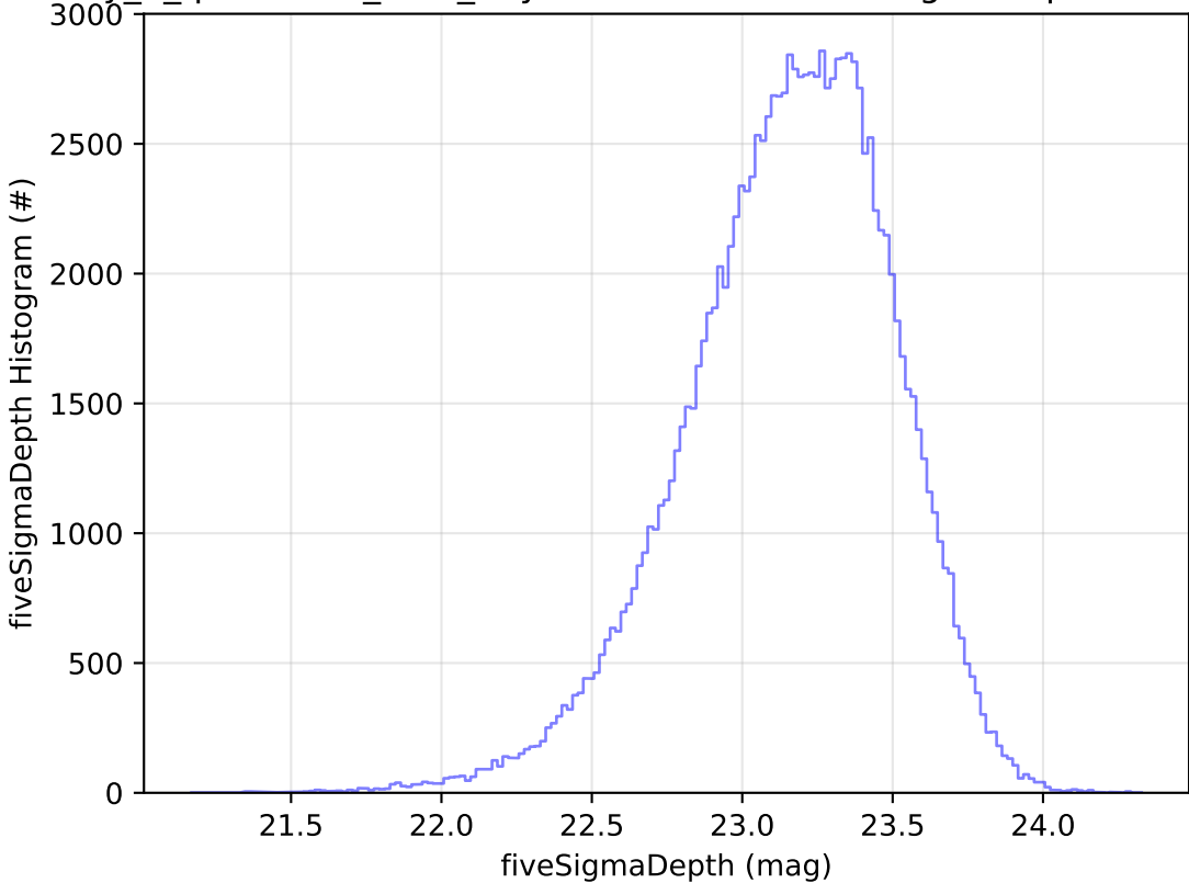
early_u_fpextra3.0_v3.4_10yrs WFD u band: fiveSigmaDepth Histogram
