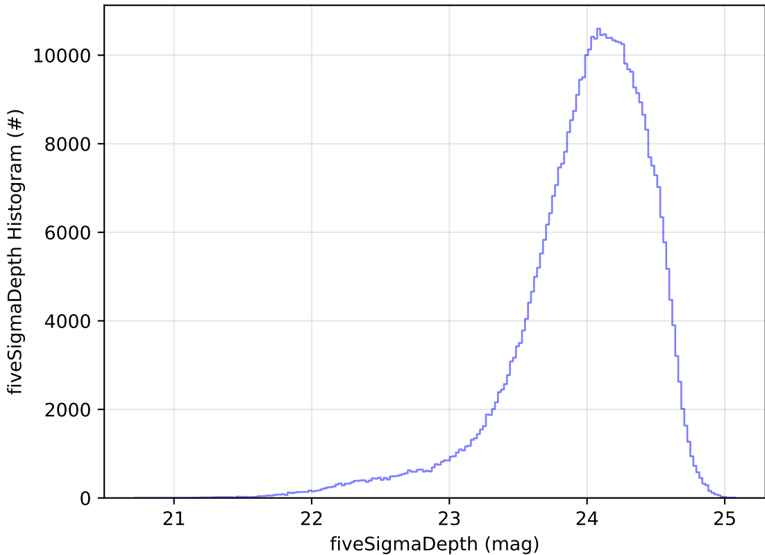
early_u_fpextra3.0_v3.4_10yrs WFD r band: fiveSigmaDepth Histogram
