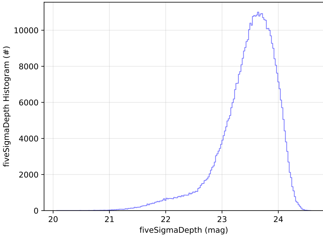
early_u_fpextra3.0_v3.4_10yrs WFD i band: fiveSigmaDepth Histogram
