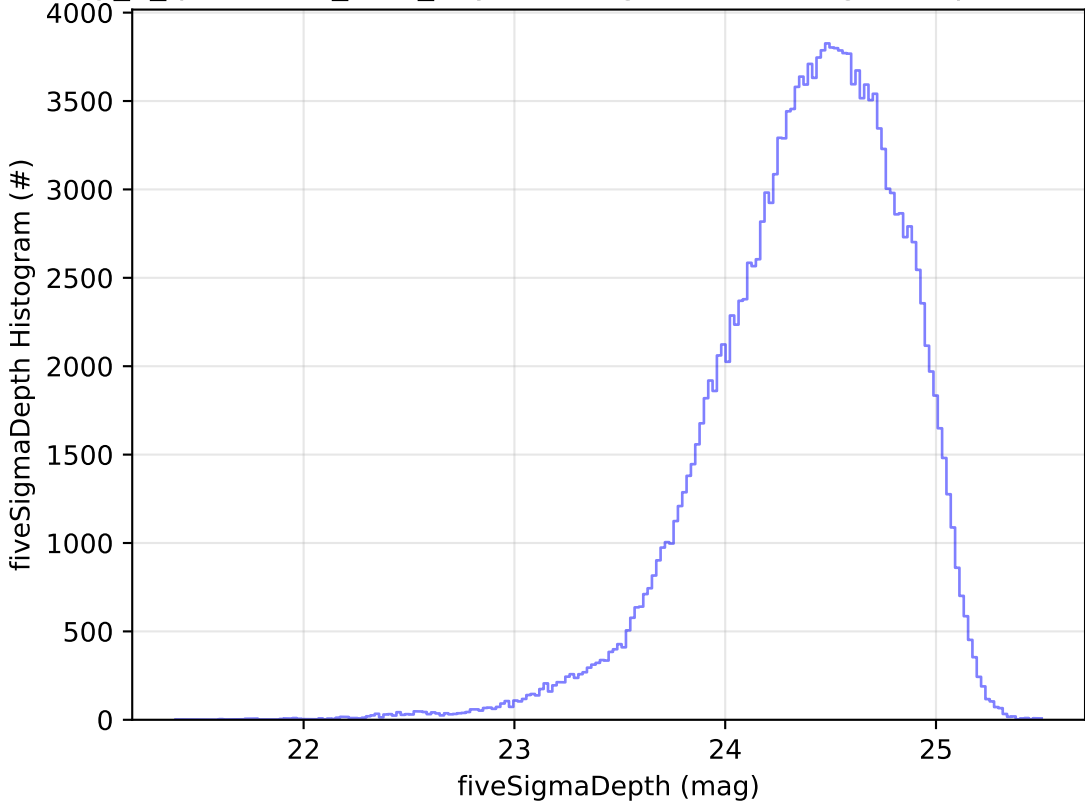
early_u_fpextra3.0_v3.4_10yrs WFD g band: fiveSigmaDepth Histogram
