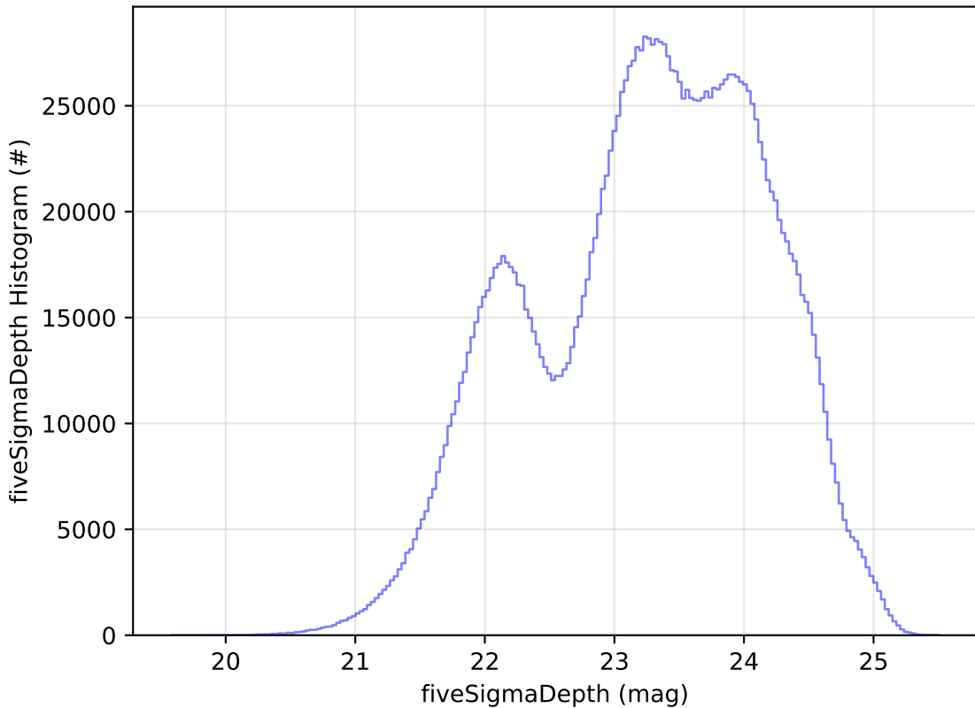
early_u_fpextra3.0_v3.4_10yrs WFD all bands: fiveSigmaDepth Histogram
