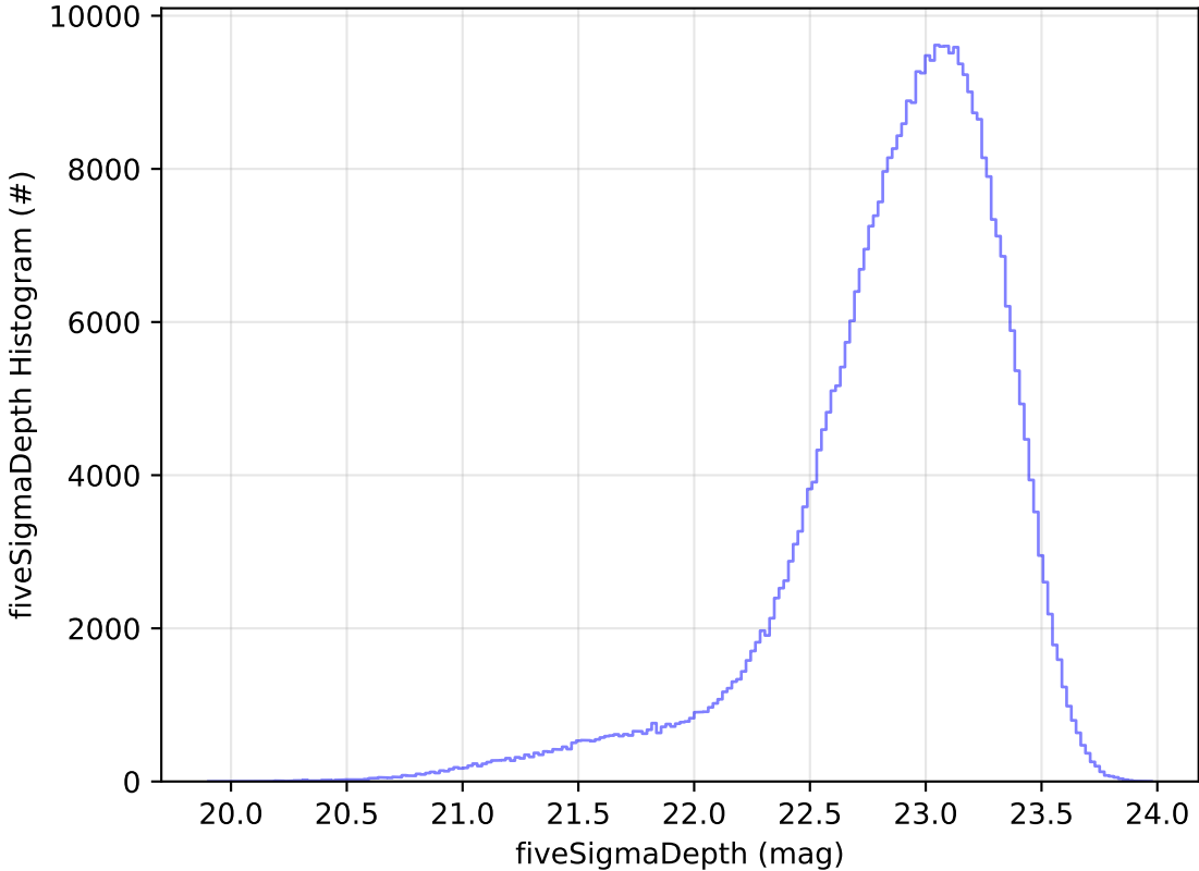
early_u_fpextra3.0_v3.4_10yrs All sky z band: fiveSigmaDepth Histogram
