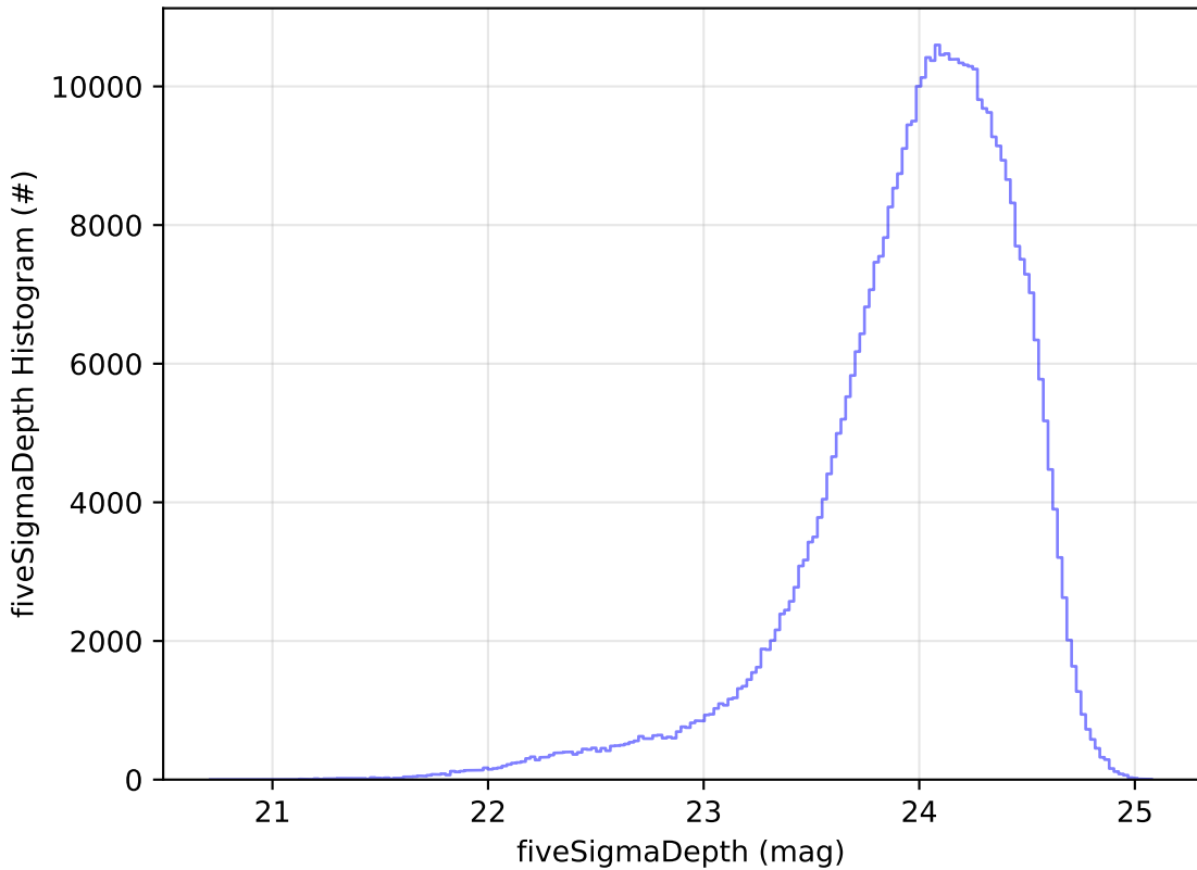
early_u_fpextra3.0_v3.4_10yrs All sky r band: fiveSigmaDepth Histogram
