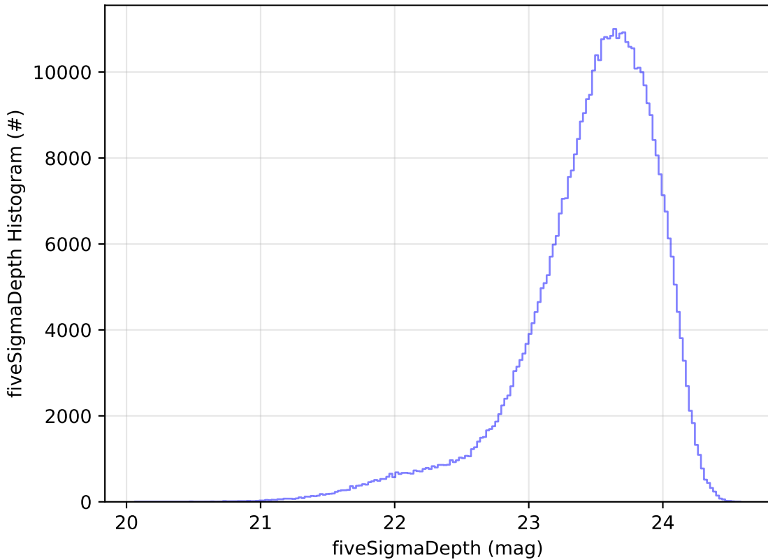
early_u_fpextra3.0_v3.4_10yrs All sky i band: fiveSigmaDepth Histogram
